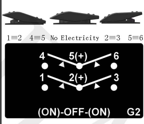
G2. (ON)-OFF-(ON)/DPDT/6P/No Lens
