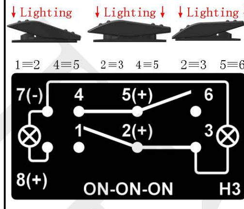
H3. ON-ON-ON/DPTT/8P/Two Lens
