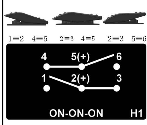
H1. ON-ON-ON/DPTT/6P/No Lens
