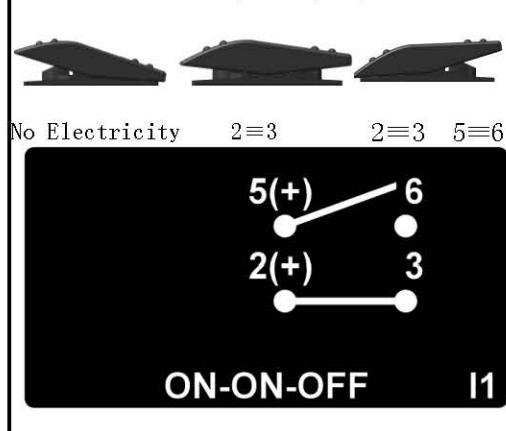
I1. ON-ON-OFF/DPDT/4P/No Lens
