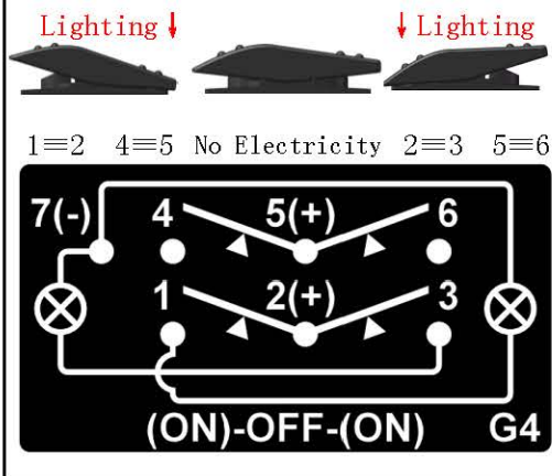
G4. (ON)-OFF-(ON)/DPDT/7P/Two Lens
