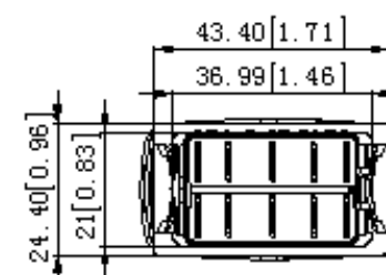
A4: 10 TERMINAL BASE
