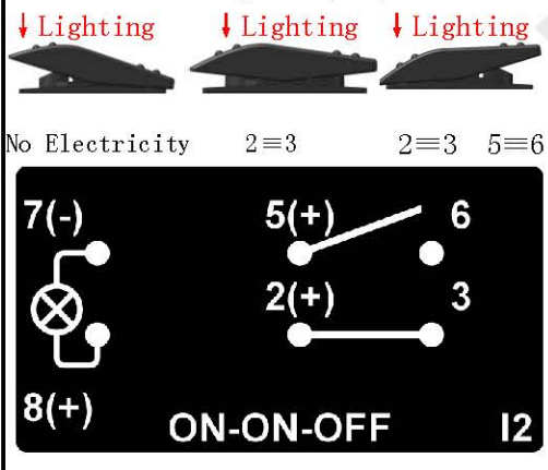
I2. ON-ON-OFF/DPDT/6P/One Lens
