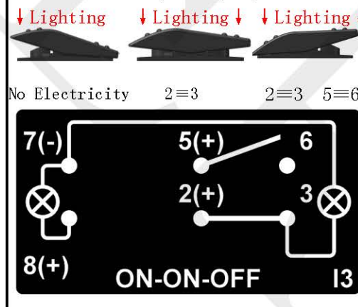
I3. ON-ON-OFF/DPDT/6P/Two Lens
