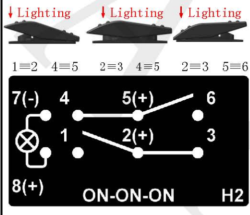
H2. ON-ON-ON/DPTT/8P/One Lens
