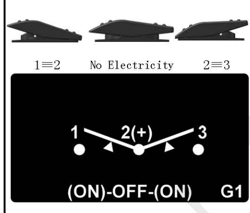
G1. (ON)-OFF-(ON)/SPDT/3P/No Lens
