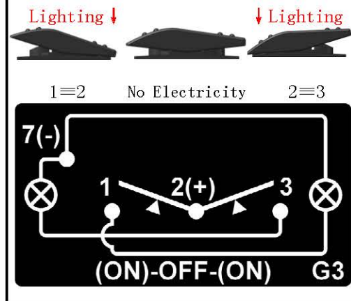
G3. (ON)-OFF-(ON)/SPDT/4P/Two Lens
